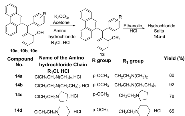
Scheme 4. Synthesis of phenolic derivatives 14a–d .
