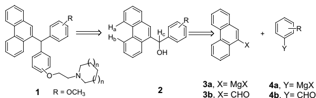
Scheme 1. Retrosynthesis of target compounds.
