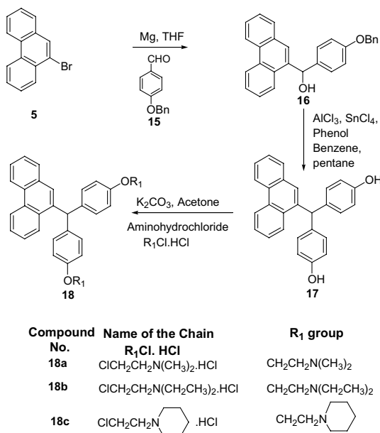
Scheme 5. Synthesis of phenolic derivatives 18a–c.
