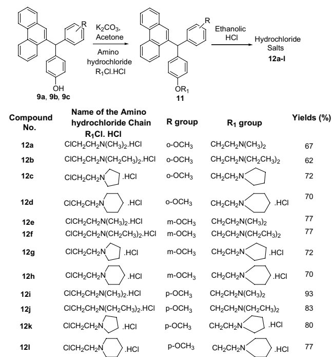
Scheme 3. Synthesis of phenolic derivatives 12a–l .
