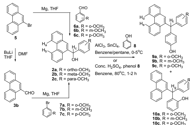
Scheme 2. Synthesis of carbinols.
